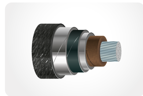
← Cables with paper-oil insulation
