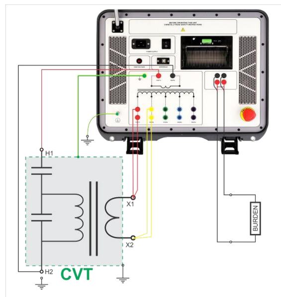
Connecting CVA500 to a CVT – secondary winding resistance test and insulation resistance test
