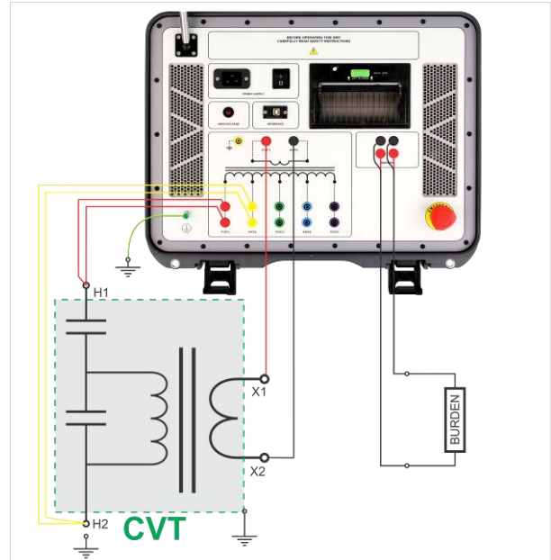
Connecting CVA500 to a CVT–turns ratio test
